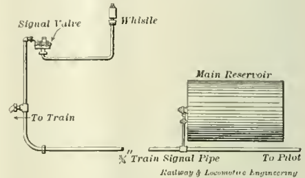
FIG. 2.—SIGNAL PIPING.
